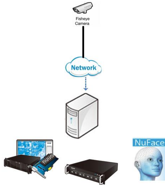
Figure 1: testing architecture
